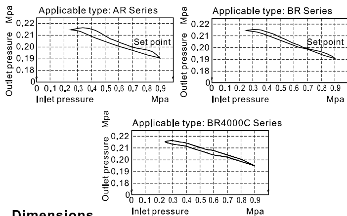
Pressure chart
